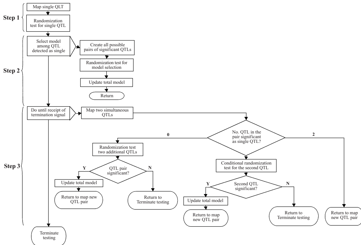
Fig. 1. Flow chart for the randomization testing strategy used to detect multiple QTLs.
