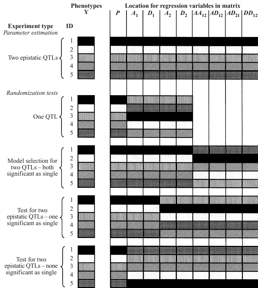
Fig. 2. One possible data permutation in four different types of randomization test based on a dataset of five individuals (ID 1–5). The randomization tests are for: 1, one QTL; 2, model selection between an epistatic and an additive/dominance model; 3, a second QTL interacting with a QTL already in the model; 4, two additional interacting QTLs. Each column represents a parameter in the model and each row represents an individual entry. The shadings indicates the individual origins of the regression variables.
